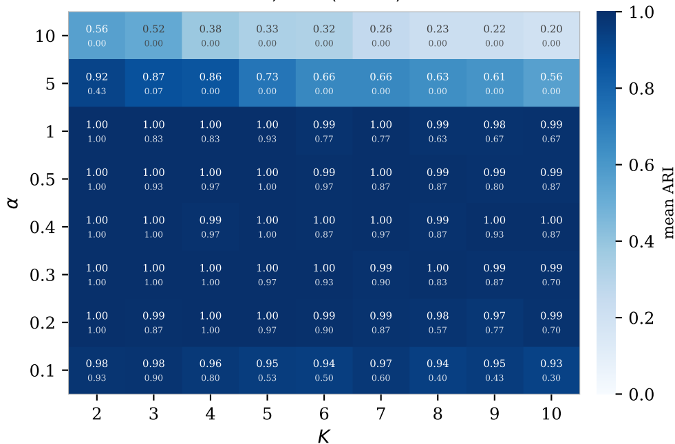
K -medoids, n = 1000 , N = 800 mean ARI, and \hat{P}(\text{ARI} = 1) below
