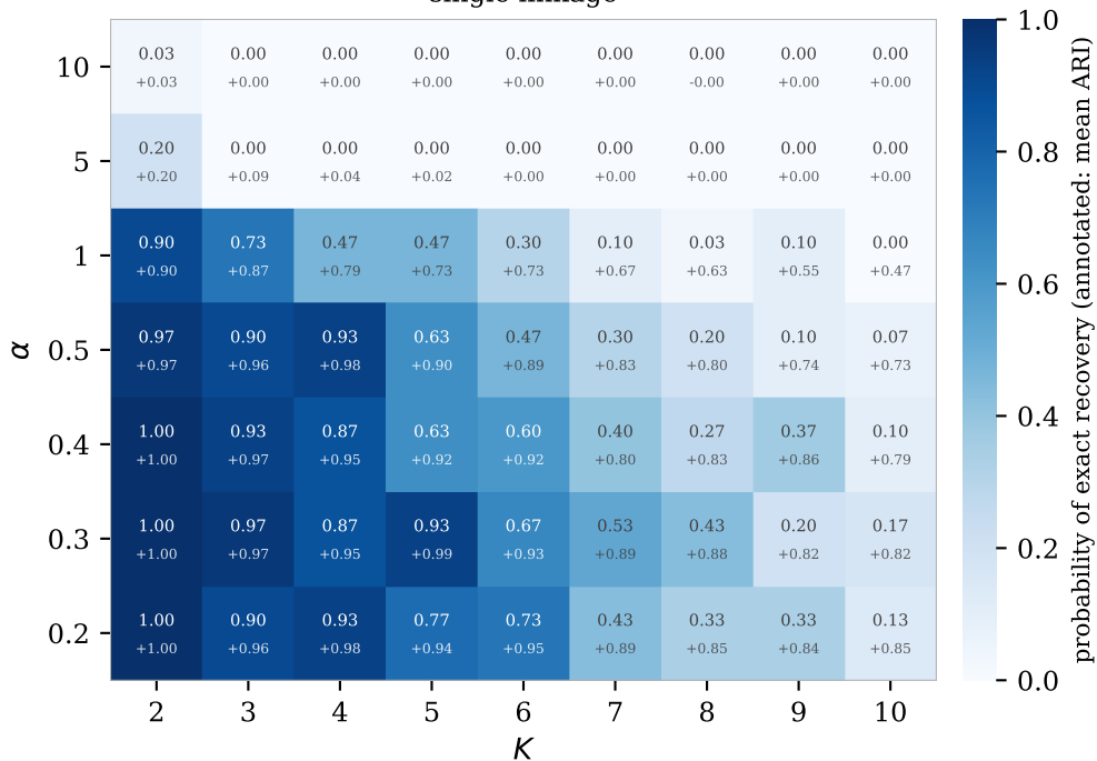
single linkage
