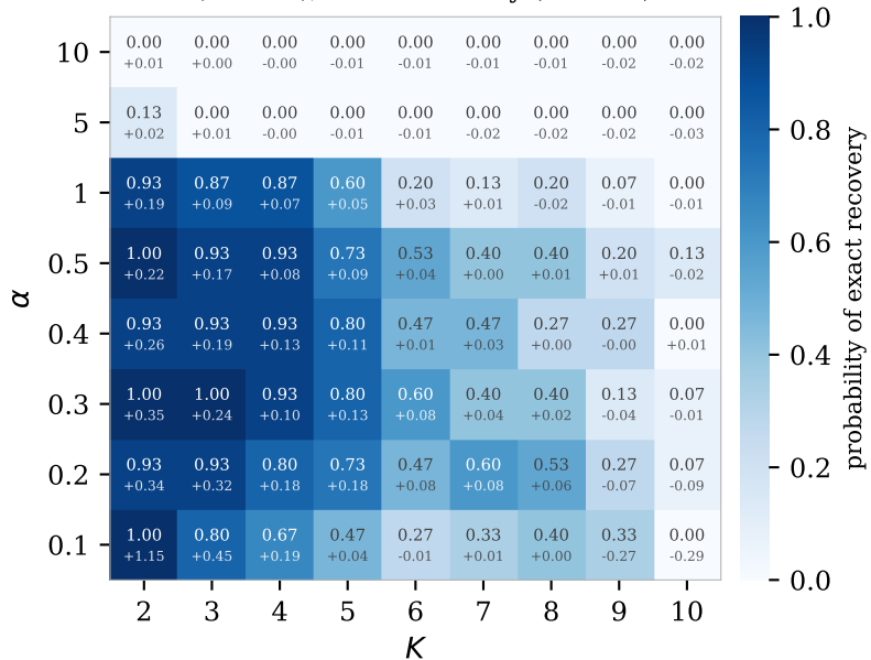
\hat{P}(\text{ARI} = 1) , exact recovery ( n = 600 )
