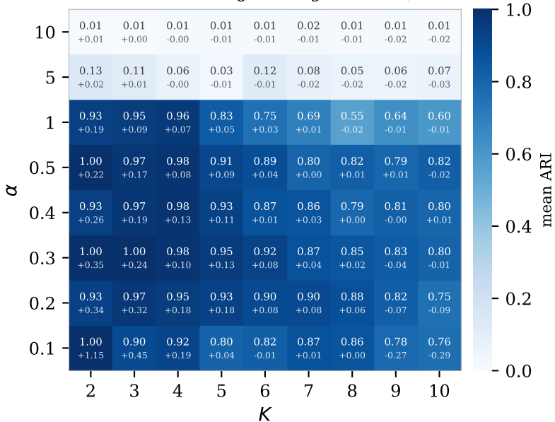
mean ARI, single linkage ( n = 600 )
