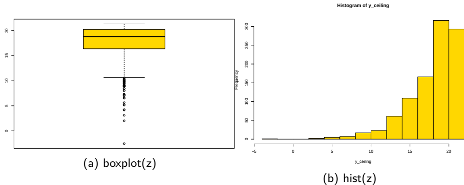
Figure 16: Boxplot vs Istogramma
