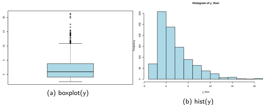
Figure 15: Boxplot vs Istogramma
