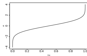
(a) Quantile
