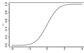
(a) Cumulata
