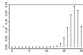
(a) \theta = .85
