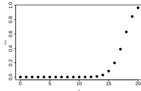
(a) \theta = .85
