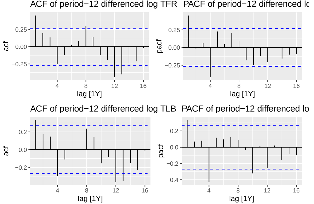
Figure 4: ACF and PACF plots of the log-first-differenced and period-12 differenced TFR and TLB series
