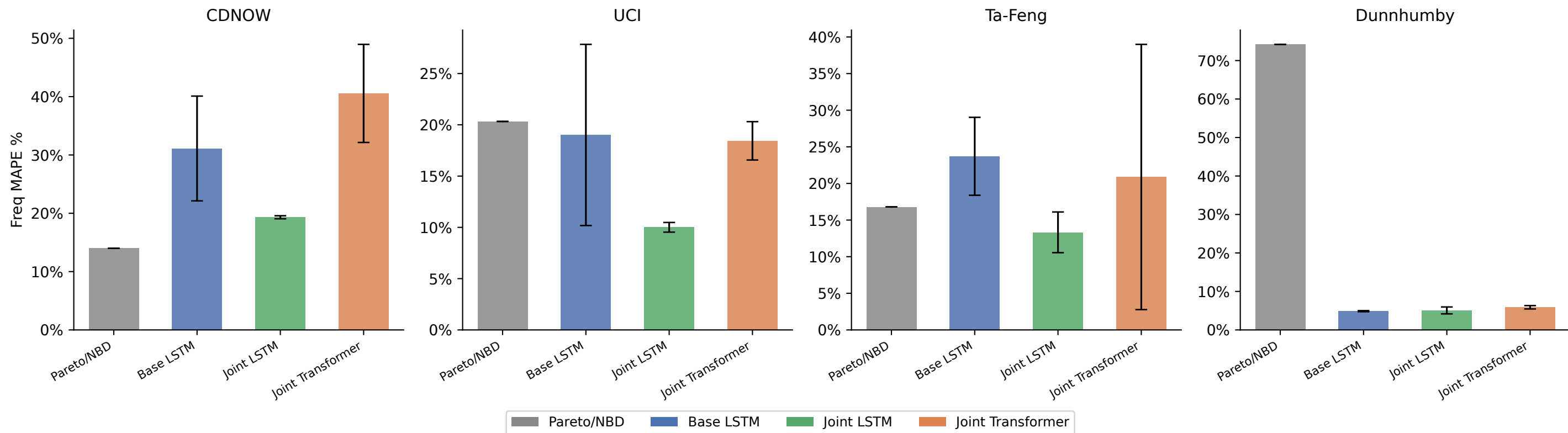
Frequency MAPE by model and dataset (lower = better) (error bars = SD across 3 seeds)
