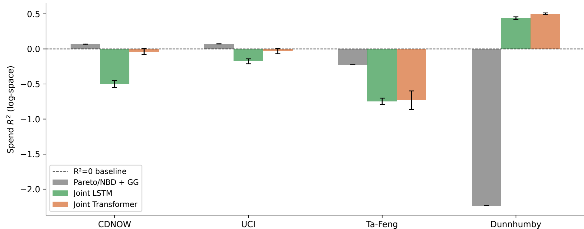
Spend prediction R^2 (log-space) across datasets (negative = worse than mean baseline)
