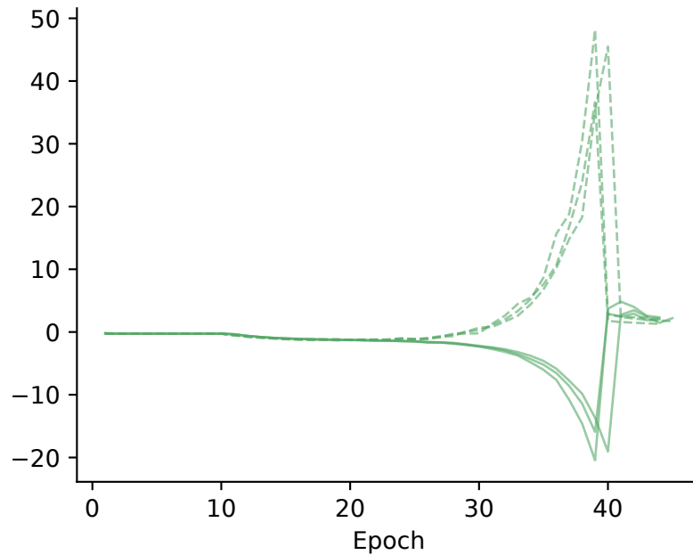
Joint LSTM
