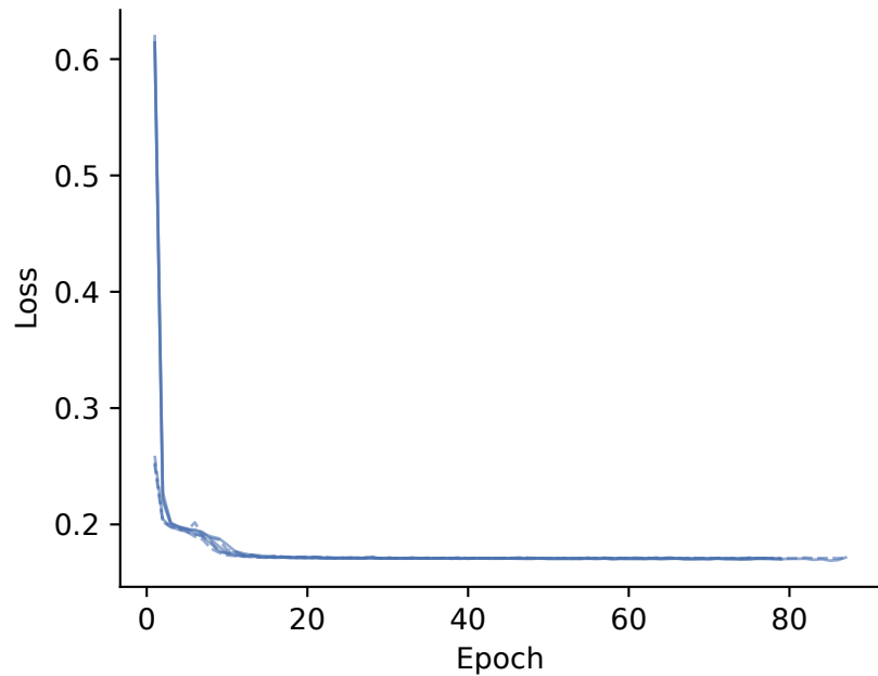
Base LSTM
