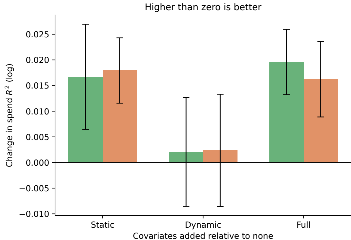
Dunnhumby covariate ablation: paired seed-wise change from no covariates (error bars = SD across three seeds)
