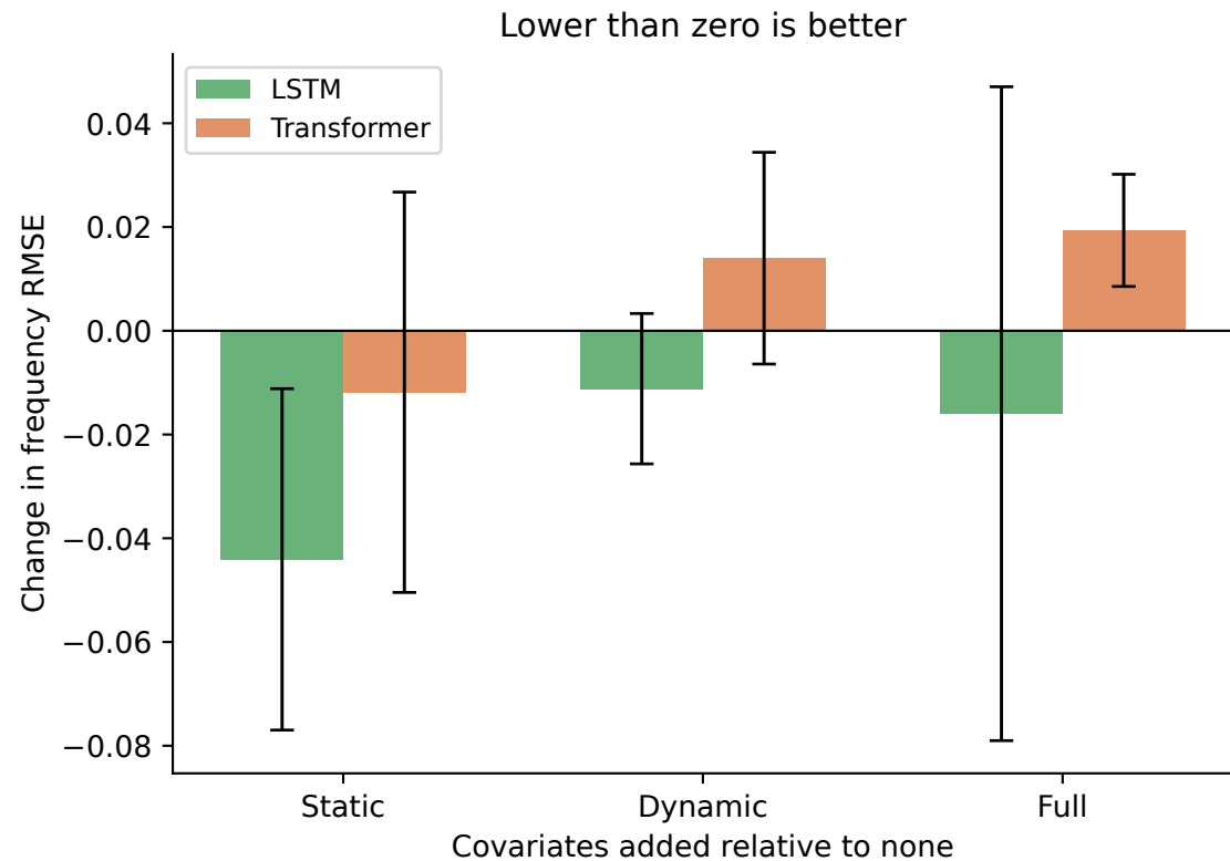
Dunnhumby covariate ablation: paired seed-wise change from no covariates (error bars = SD across three seeds)
