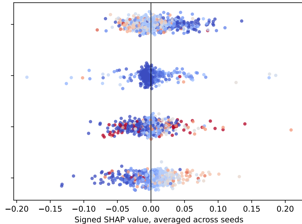
Conditional log1p-spend
