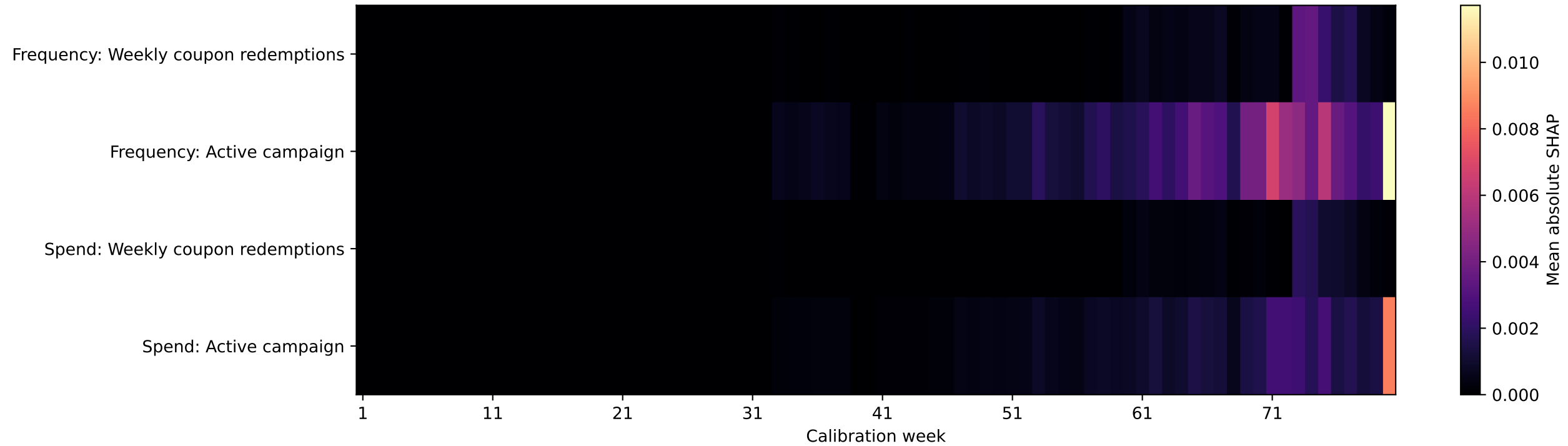
TRANSFORMER mean absolute weekly dynamic SHAP
