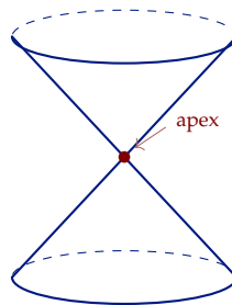
Quadric cone V(xy - z^2) \subset \mathbb{A}^3 singular locus = apex (codim 2) normal
