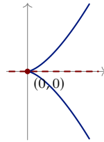
Cusp C : y^2 = x^3
