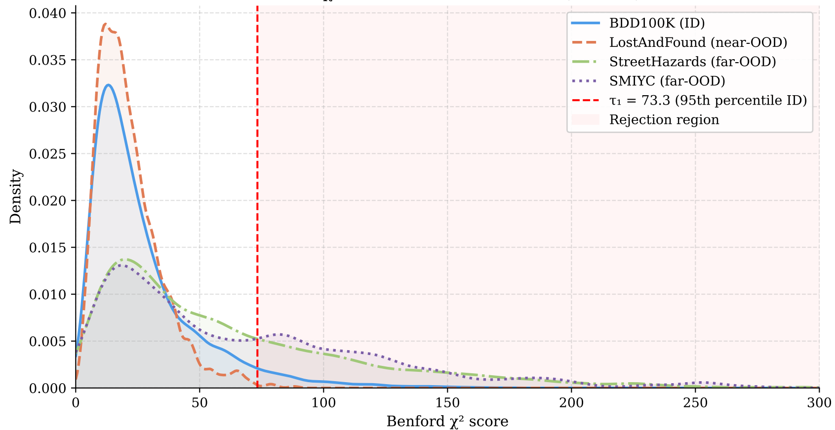
Benford \chi^2 Distributions — ID vs OOD (DINOv2)
