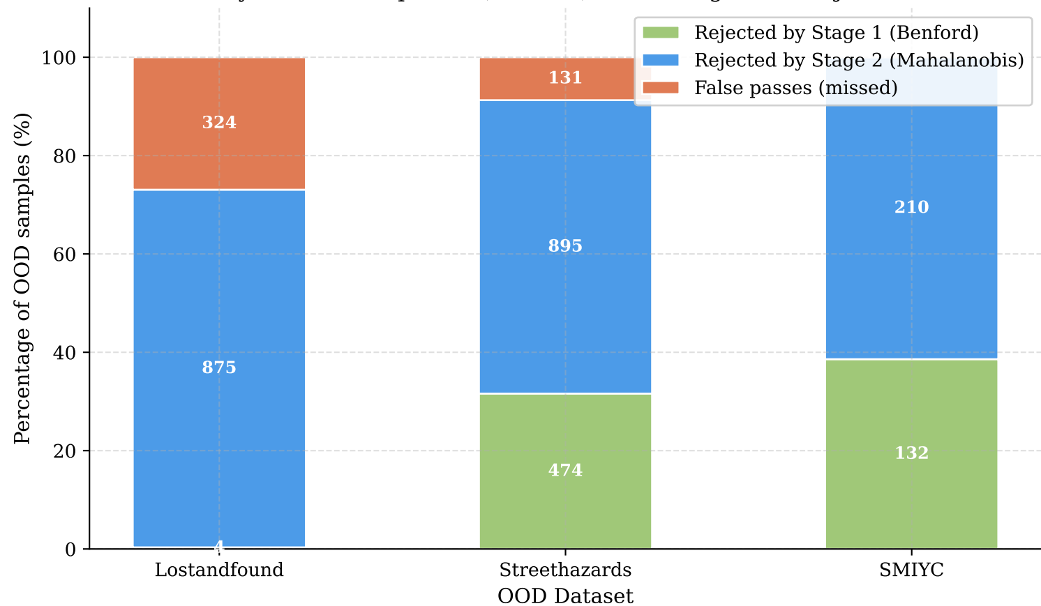
Hybrid Gatekeeper V3 (DINOv2) — Per-Stage OOD Rejection
