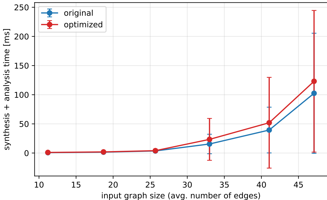
Computation time: original vs. optimized
