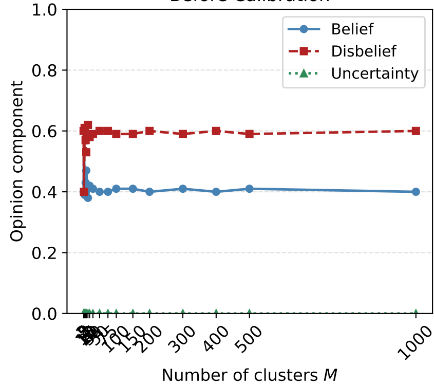
CIFAR — Trust opinion vs. number of clusters (epoch 100) Before Calibration After Calibration
