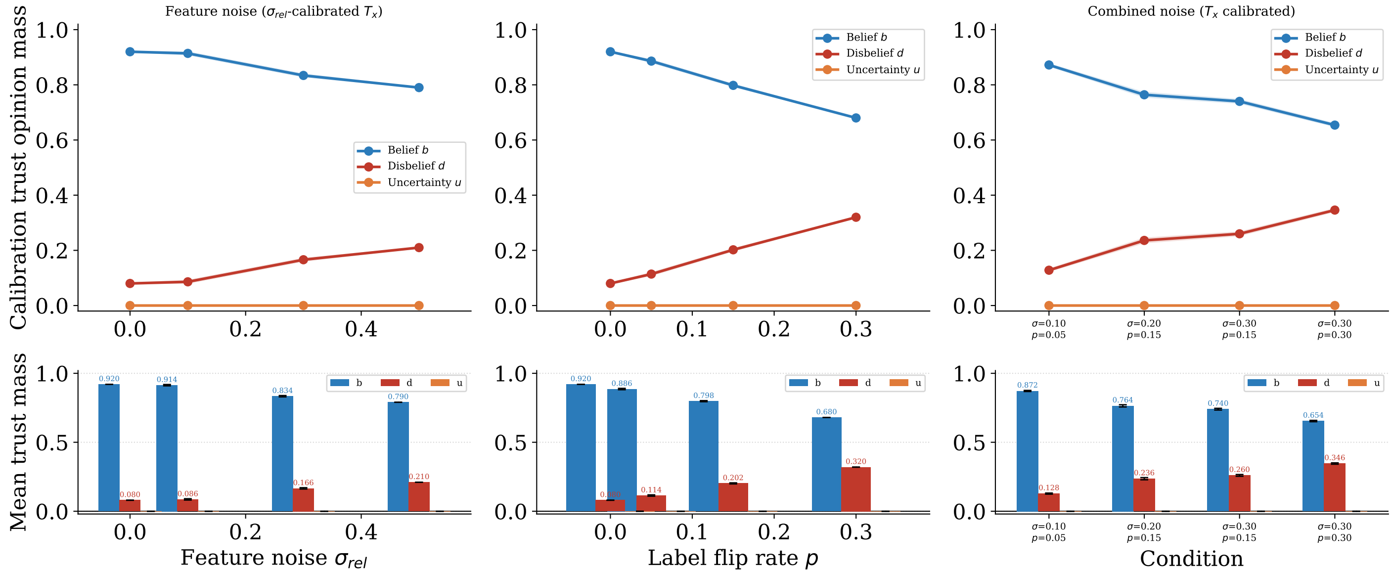
Calibration Trust of trained NNs across noise conditions (mean \pm std over 5 runs, M=10 bins, W=2, BPQ + cumulative fusion)
