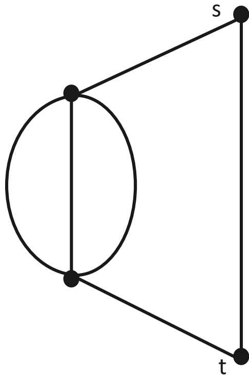
Reduction 1
