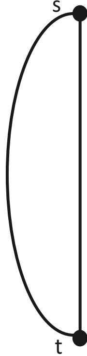
Reduction 3
