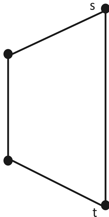
Reduction 2
