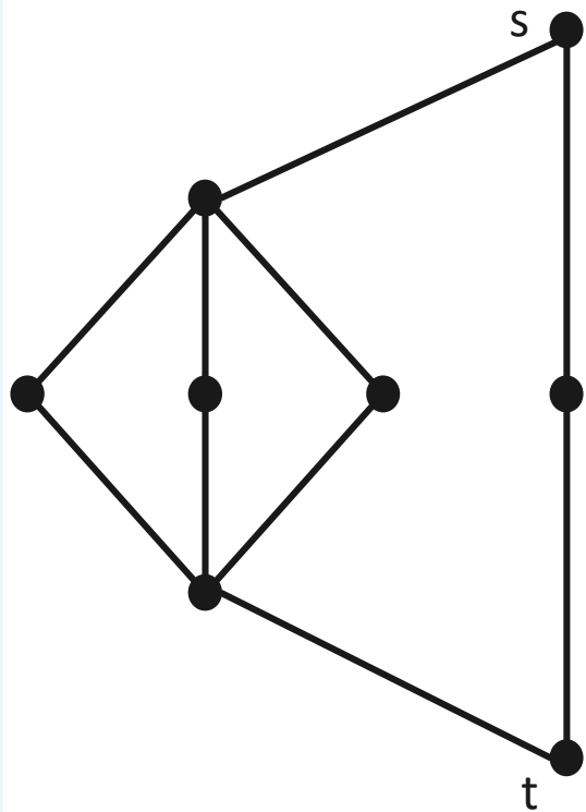
SP-graph
