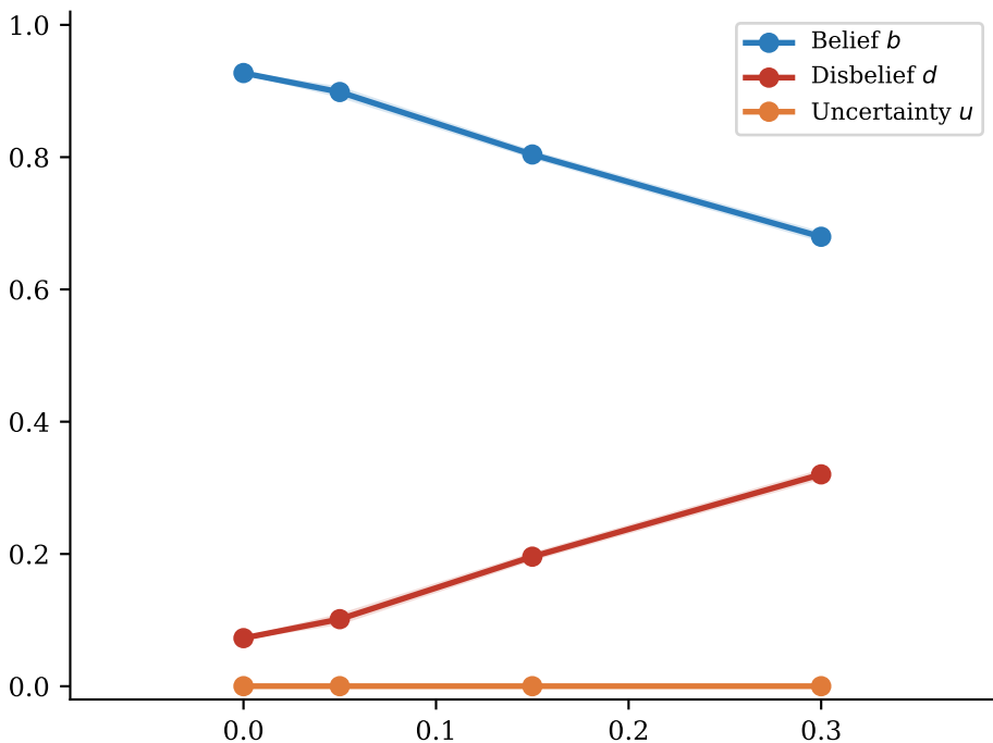
Label noise (trusted \mathcal{T}_x )
