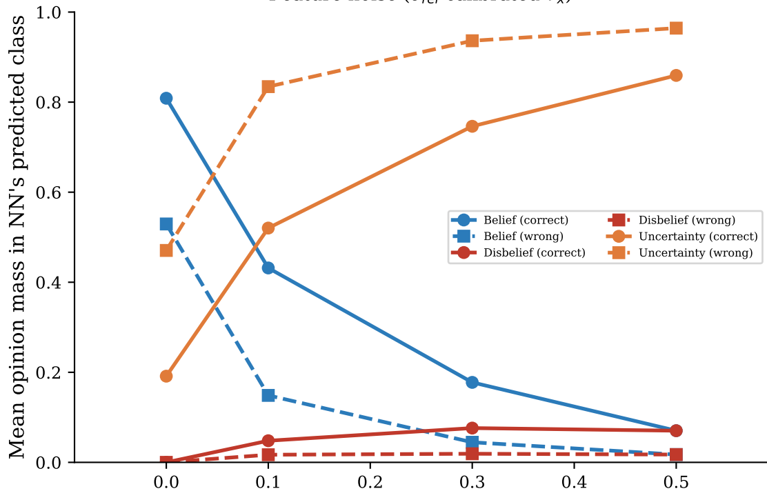
Feature noise ( \sigma_{rel} -calibrated T_x )
