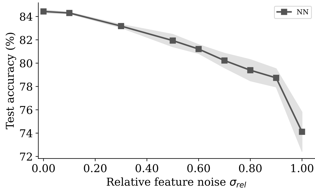
NN: feature measurement noise
