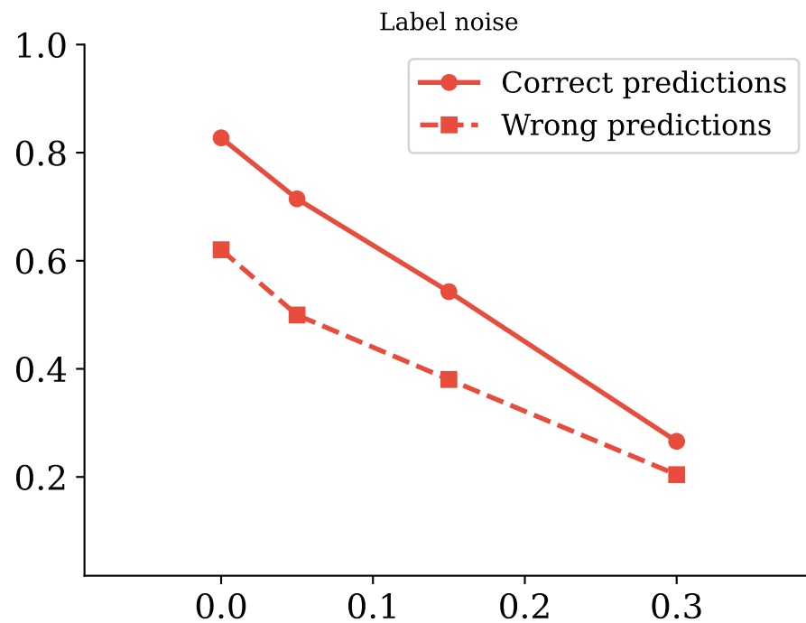
PaTAS signal: correct vs. wrong predictions
