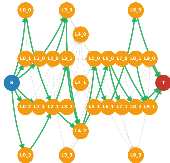
G' — Optimized 33 / 75 edges (44%) is_dspg=True
