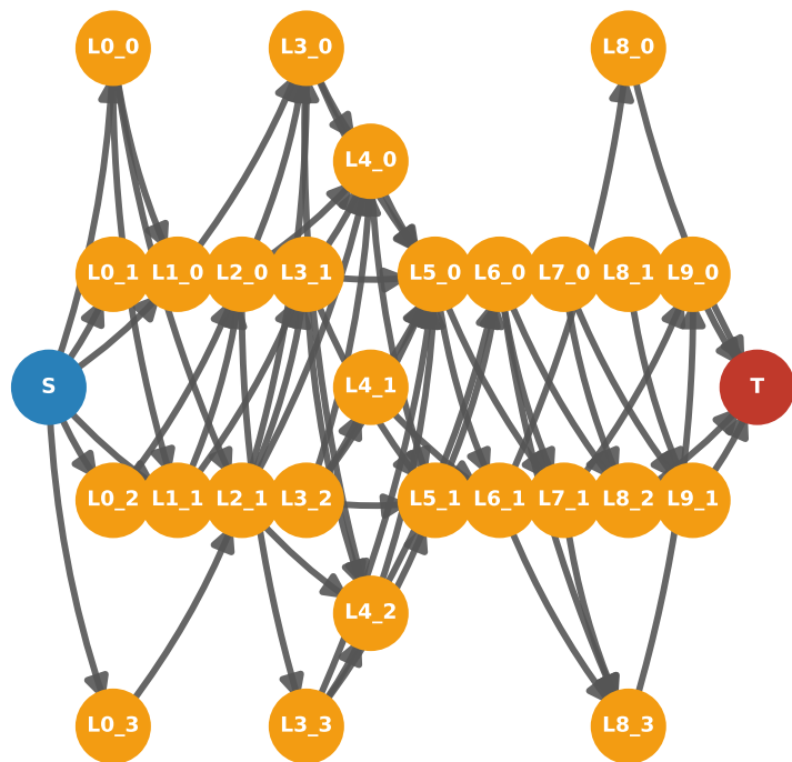
Input graph G 29 nodes · 75 edges
