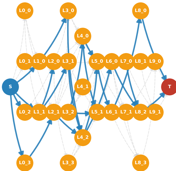
G' — Original NNL 28 / 75 edges (37%) is_dspg=False
