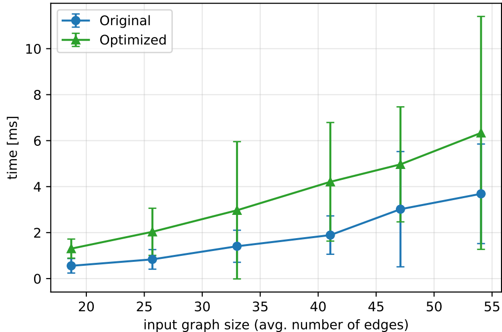
DSPG Analysis time
