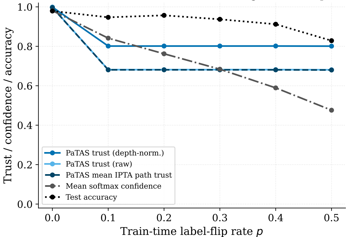
MNIST — PaTAS model trust vs. training-label corruption
