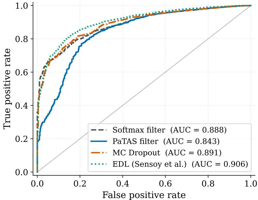
Fashion-MNIST (Mixed batch (clean + p=0.6 , 1:1)) — correct-vs-incorrect ROC
