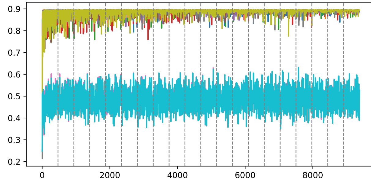
Evolution of distrust mass for fully distrusted input
