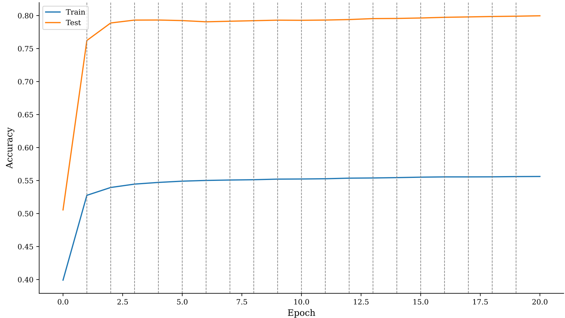
Accuracy Evolution
