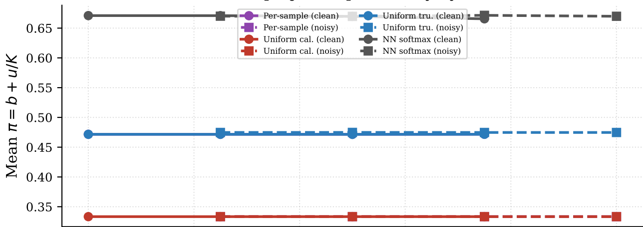
\sigma=1.00 : mean projected probability by noise status
