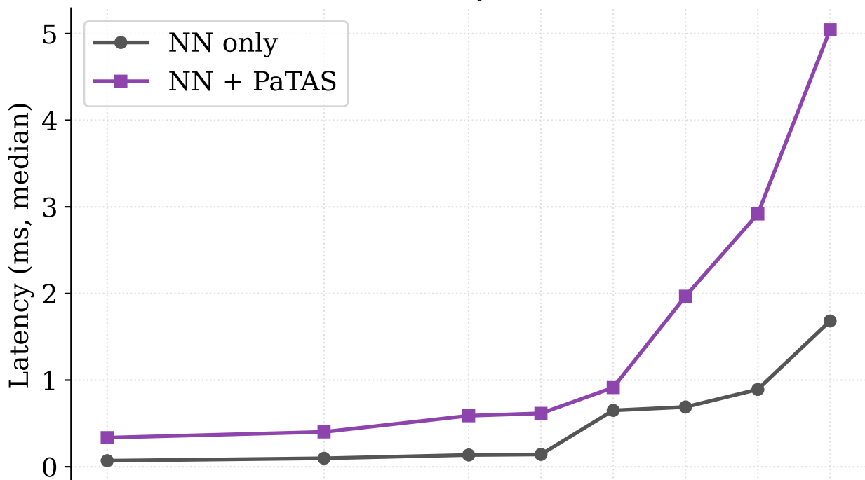
Inference latency vs batch size
