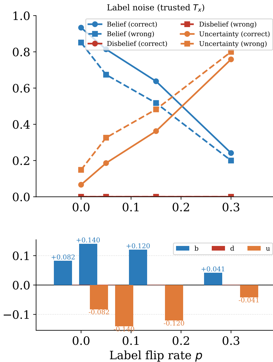
PaTAS confidence signal: opinion masses in predicted class
