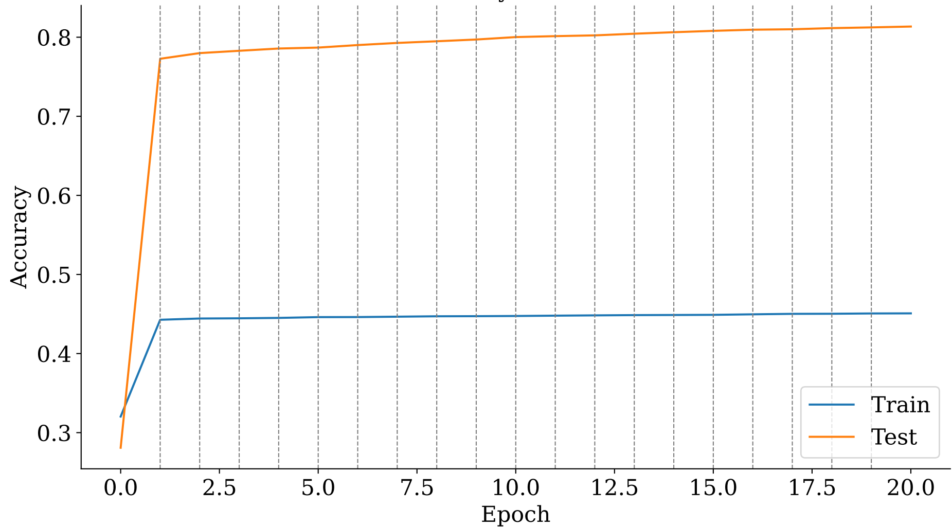
Accuracy Evolution
