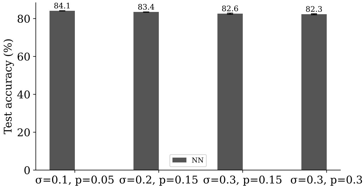
NN: combined feature + label noise
