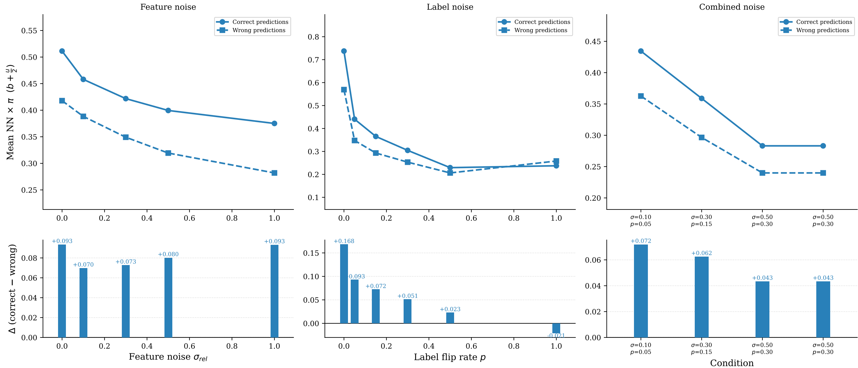
PaTAS combined signal — \text{NN} \times \pi \left(b + \frac{u}{2}\right) : correct vs. wrong predictions
