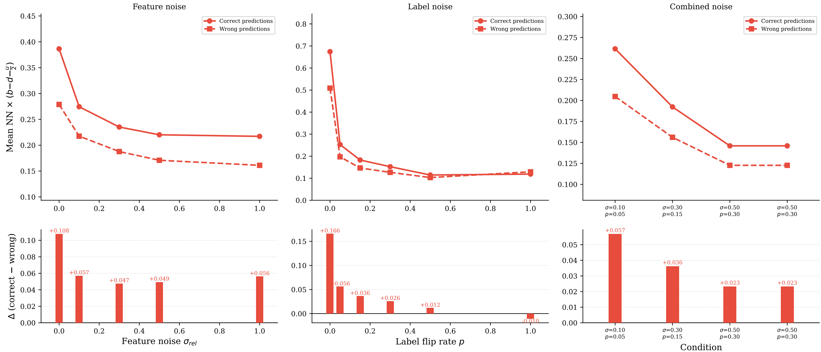
PaTAS combined signal — \text{NN} \times (b-d-\frac{u}{2}) : correct vs. wrong predictions
