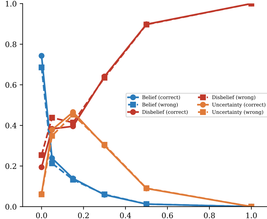
Label noise (trusted T_x )
