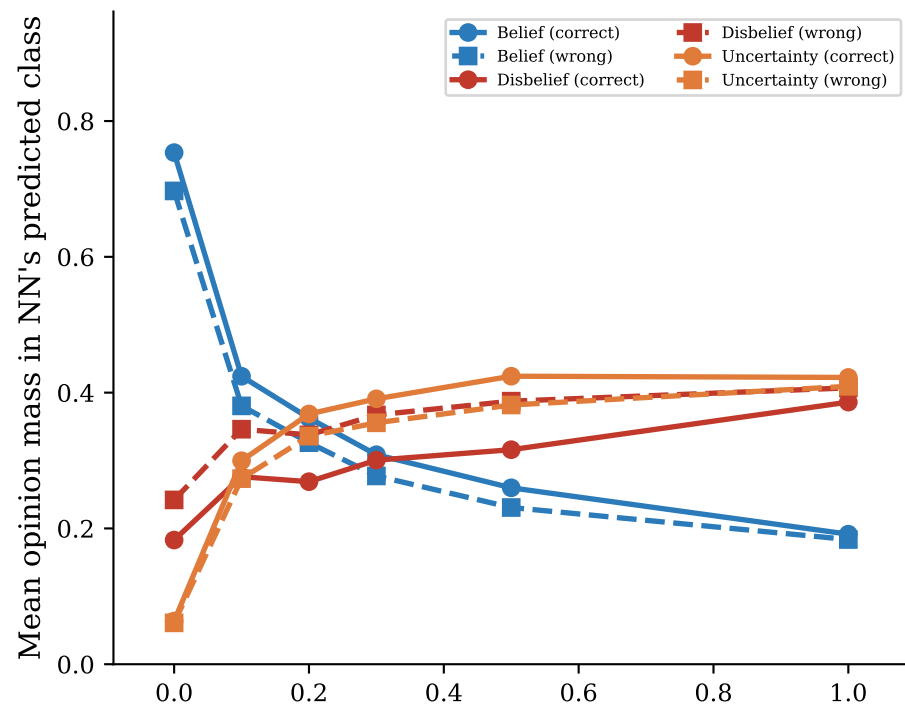
Feature noise ( \sigma_{rel} -calibrated T_x )
