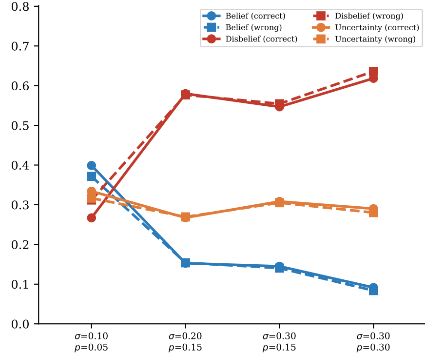
Combined noise ( T_x calibrated)
