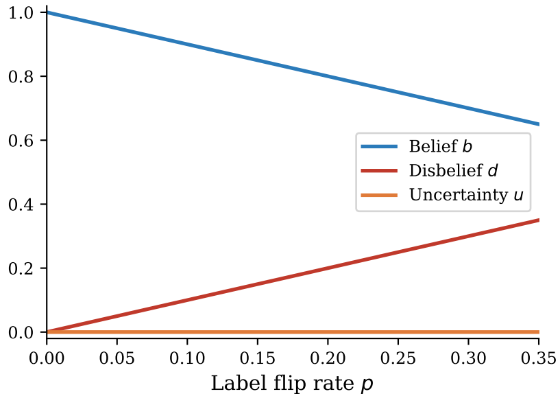
Label noise \rightarrow trust opinion
