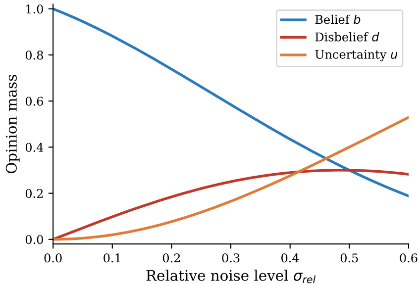
Feature noise \rightarrow trust opinion
