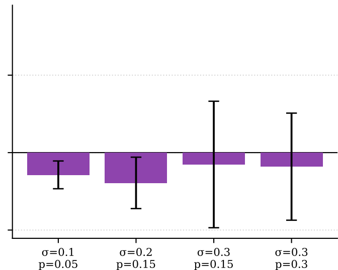
Combined noise
