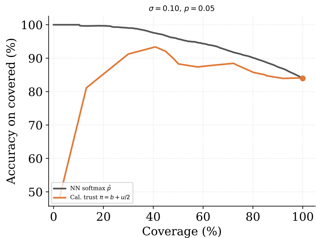
Calibration-based Coverage-Accuracy — Combined noise ( \pi = b + u/2 threshold vs. NN softmax)
