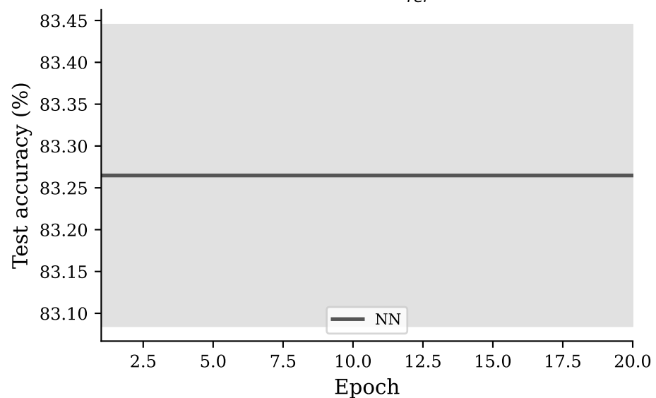
Label noise p = 0.15
