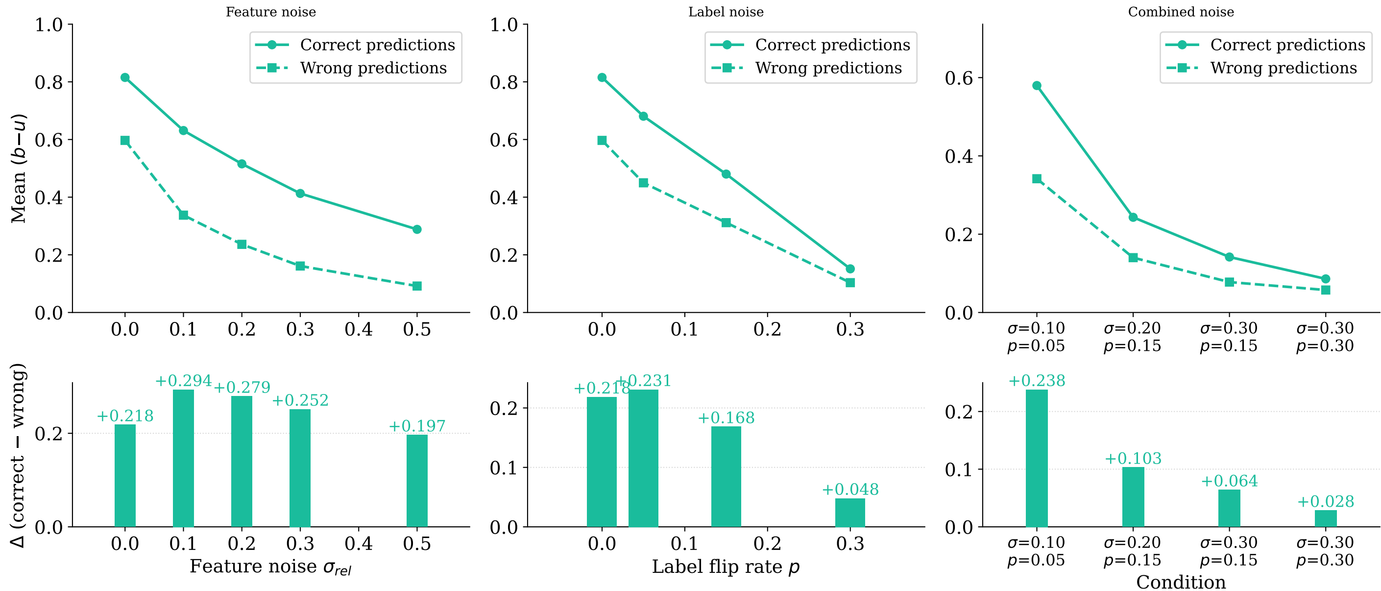
PaTAS signal: correct vs. wrong predictions
