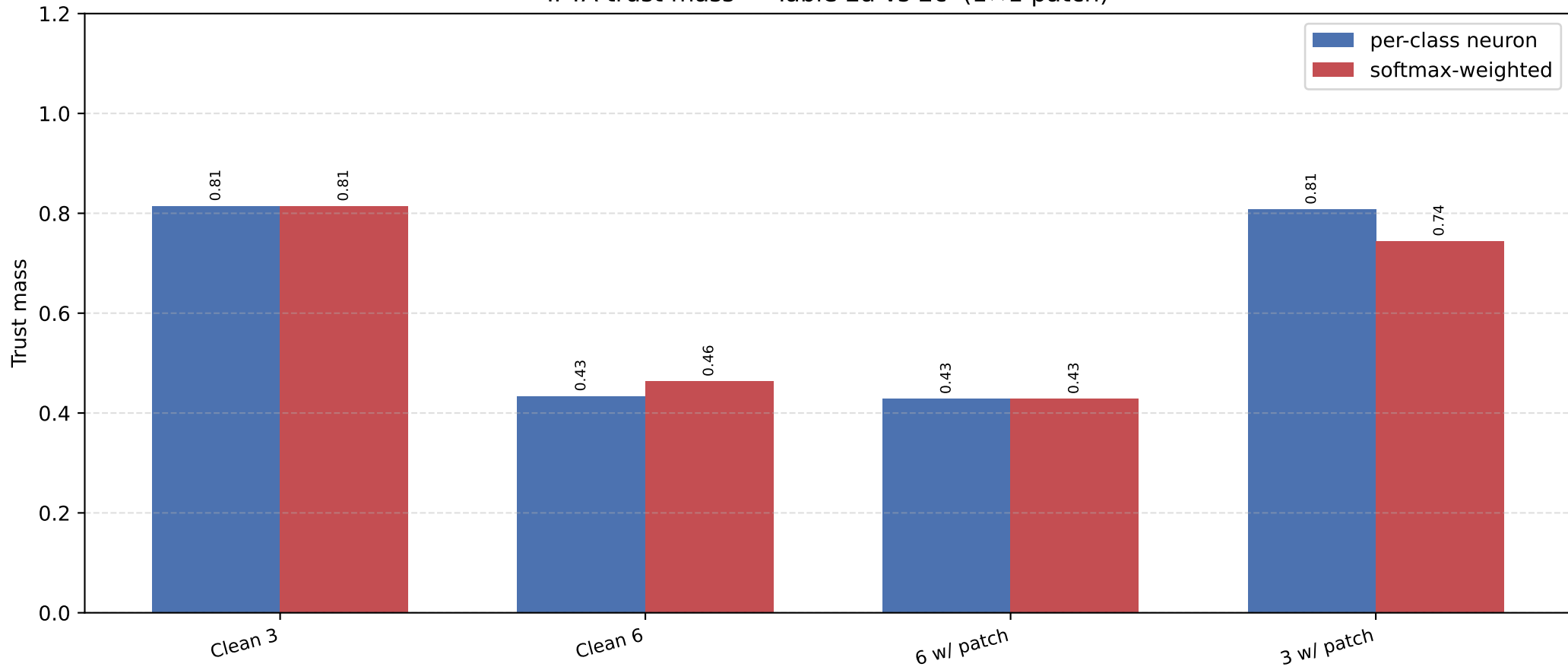
IPTA trust mass — Table 2a vs 2c (1×1 patch)
