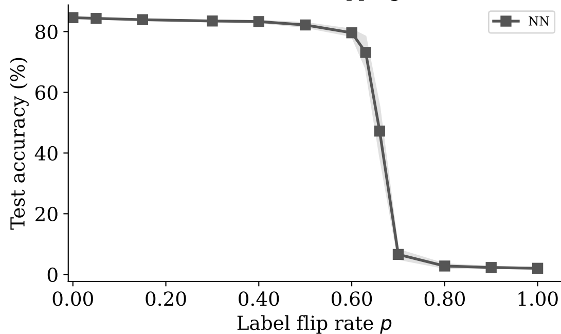
NN: label flipping
