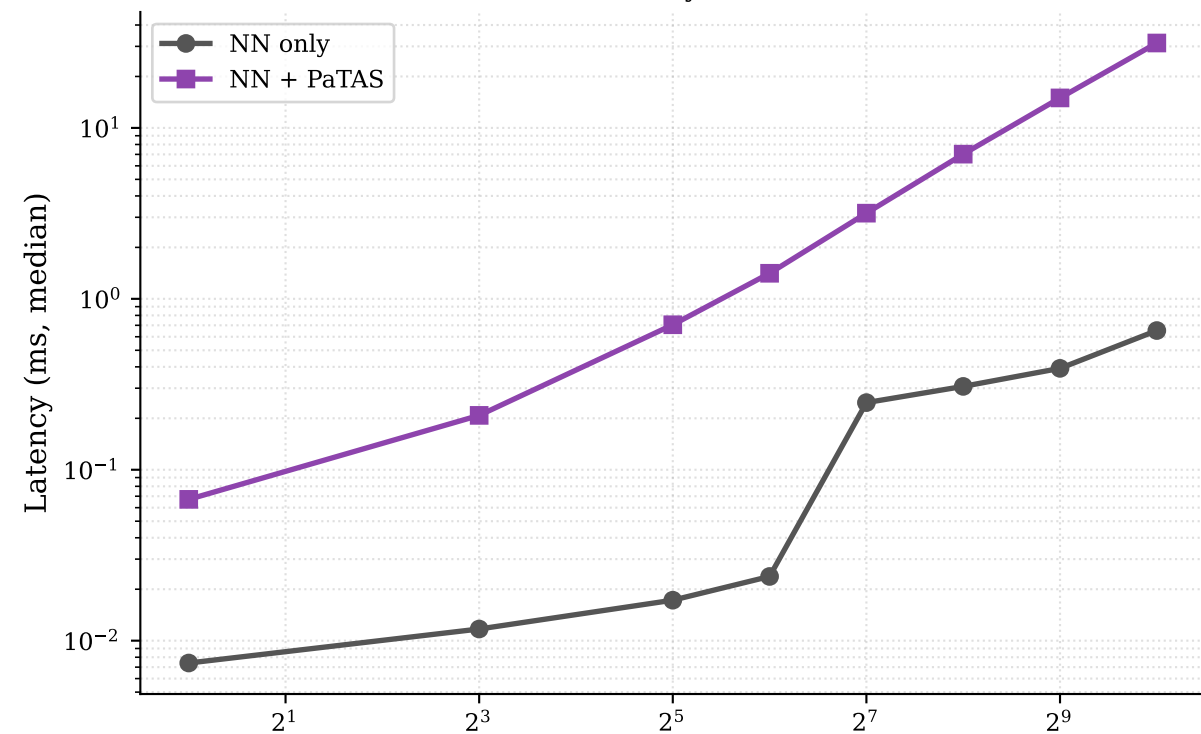
Inference latency vs batch size
