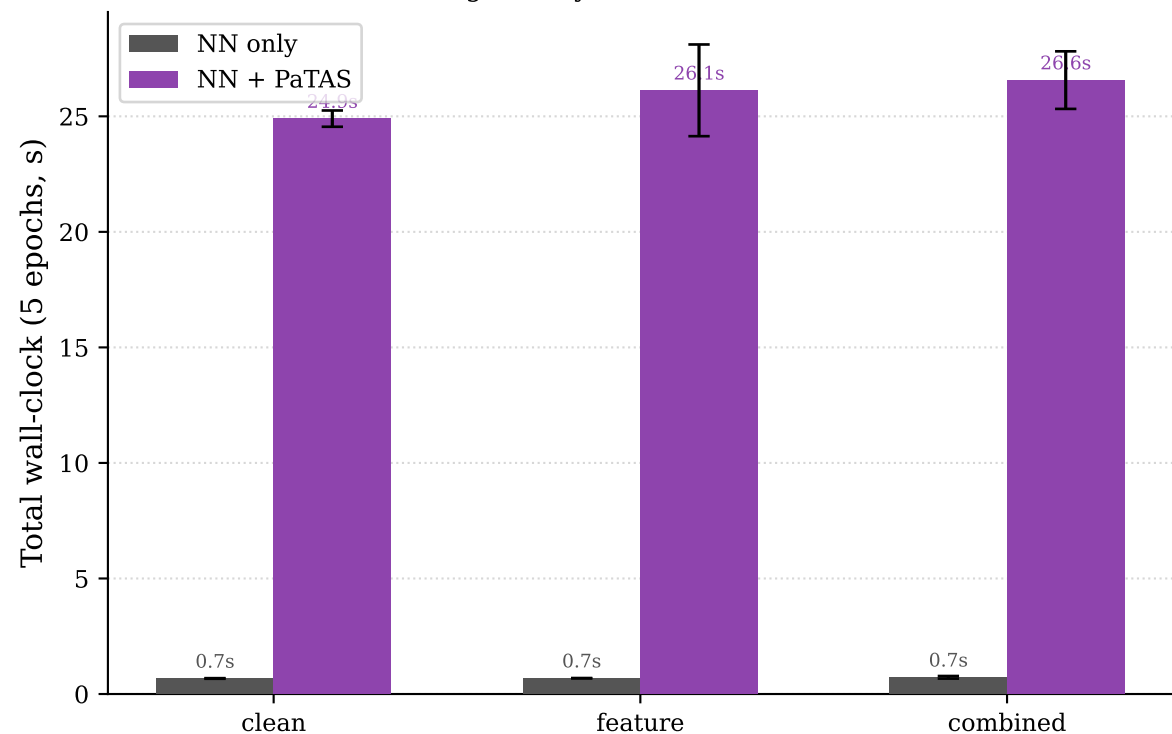
Training latency across noise conditions
