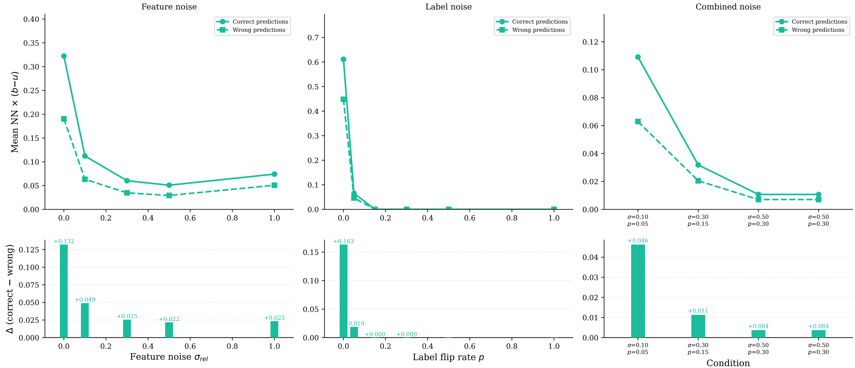
PaTAS combined signal — \text{NN} \times (b-u) : correct vs. wrong predictions
