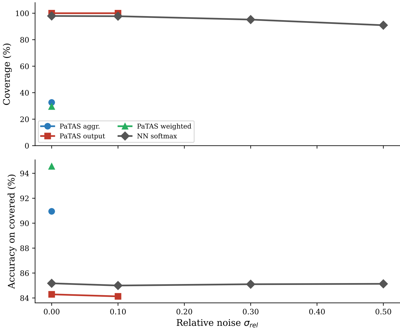
Feature noise — filter: 'b>u' ( \tau=0.500 )
