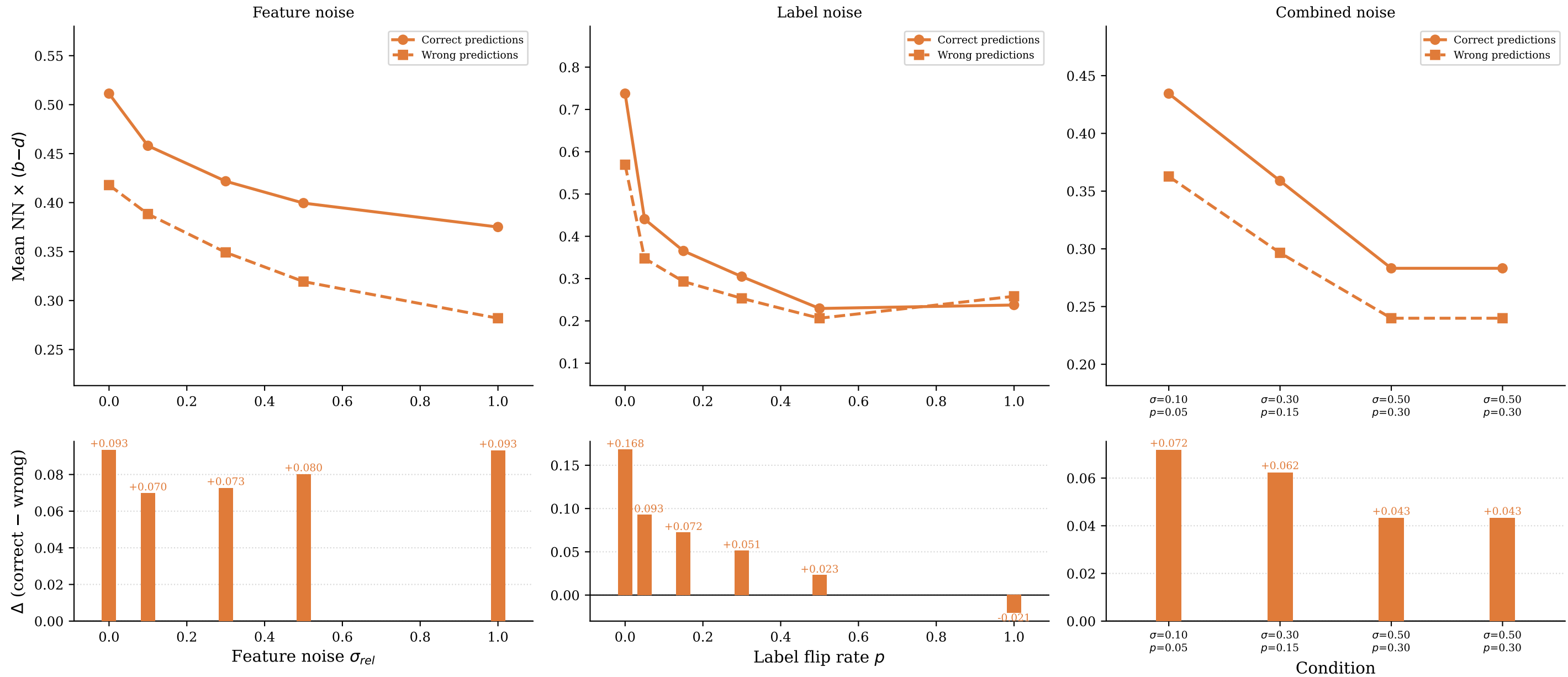
PaTAS combined signal — \text{NN} \times (b-d) : correct vs. wrong predictions
