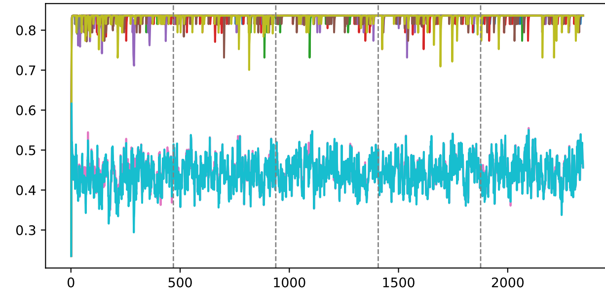
Evolution of trust mass for vacuous input
