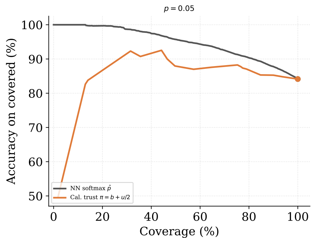
Calibration-based Coverage-Accuracy — Label noise ( \pi = b + u/2 threshold vs. NN softmax)
