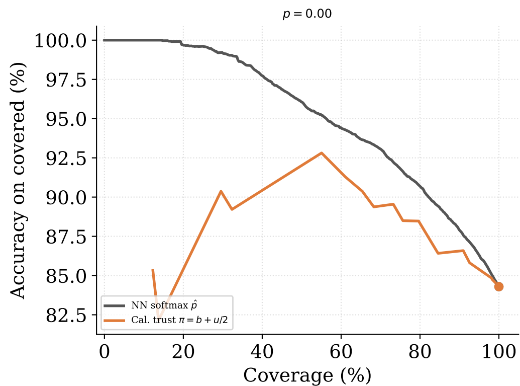
Calibration-based Coverage-Accuracy — Label noise ( \pi = b + u/2 threshold vs. NN softmax)
